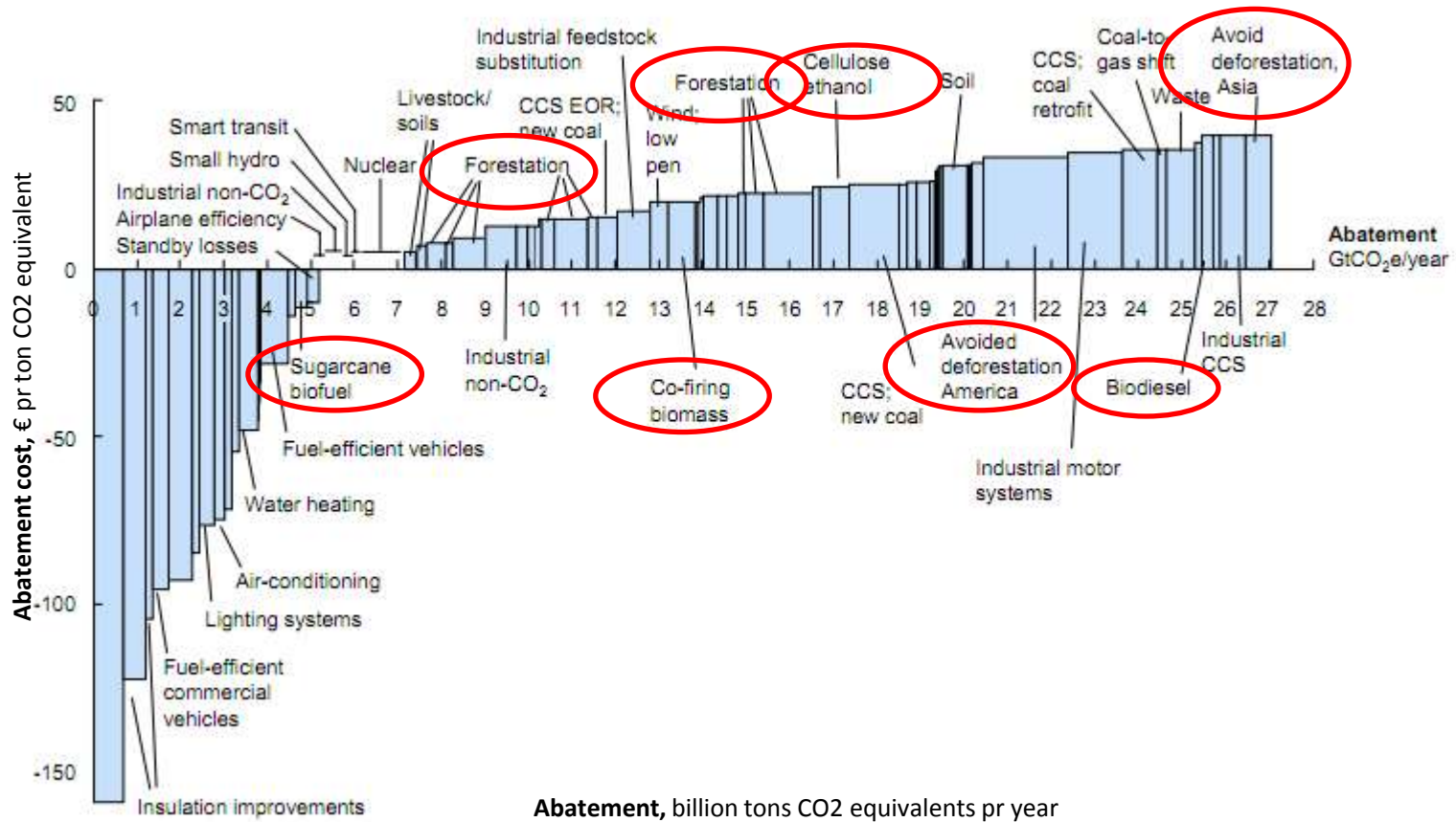
Global abatement cost curve, 2030, measured in tons of carbon dioxide and equivalent greenhouse gases (CO 2 e)
